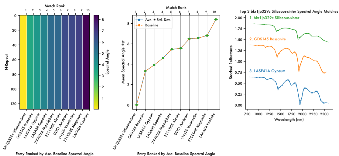
bkr1jb329c Siliceous-sinter Mean Spectral Angle Match
