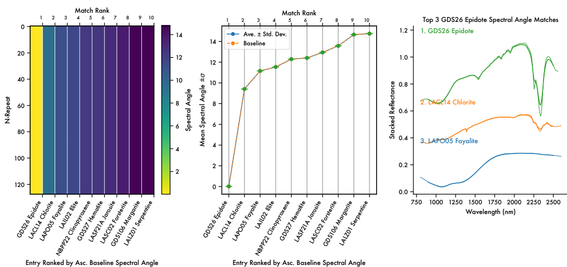
GDS26 Epidote Mean Spectral Angle Match
